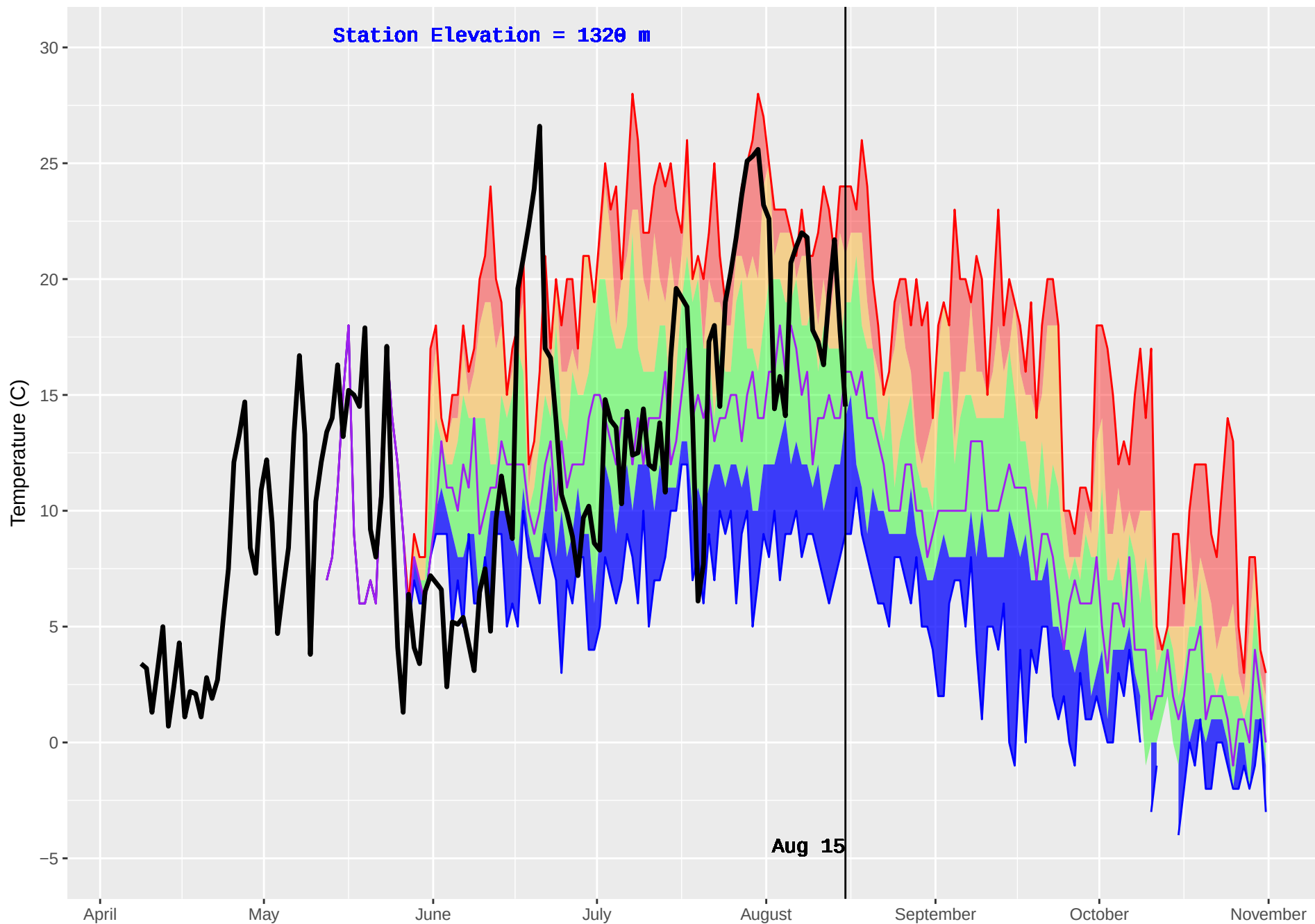
PINE CREEK (938) : Historical (2006–2016) and Current (2018) Daily Temperature
