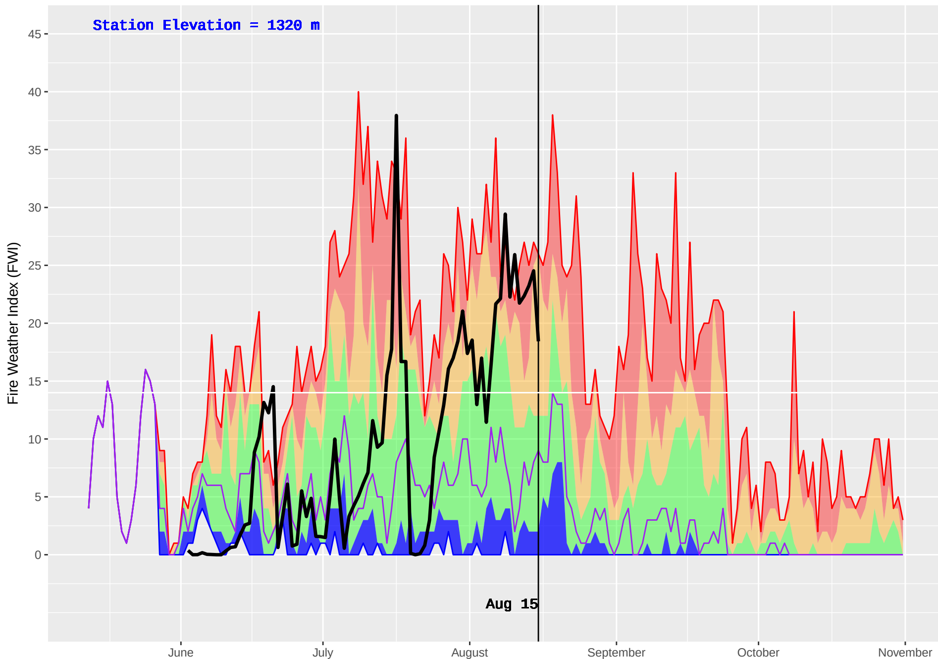
PINE CREEK (938) : Historical (2006–2016) and Current (2018) Daily Fire Weather Index (FWI)
