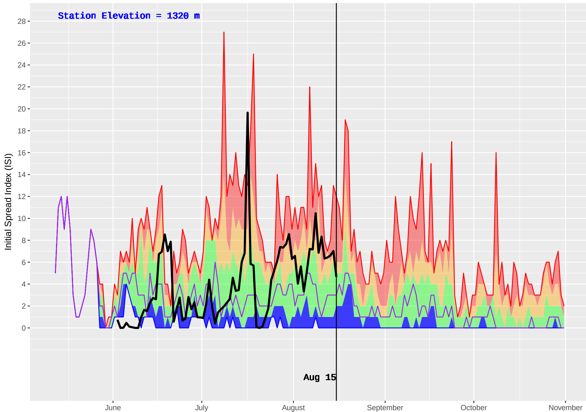
PINE CREEK (938) : Historical (2006–2016) and Current (2018) Daily Initial Spread Index (ISI)
