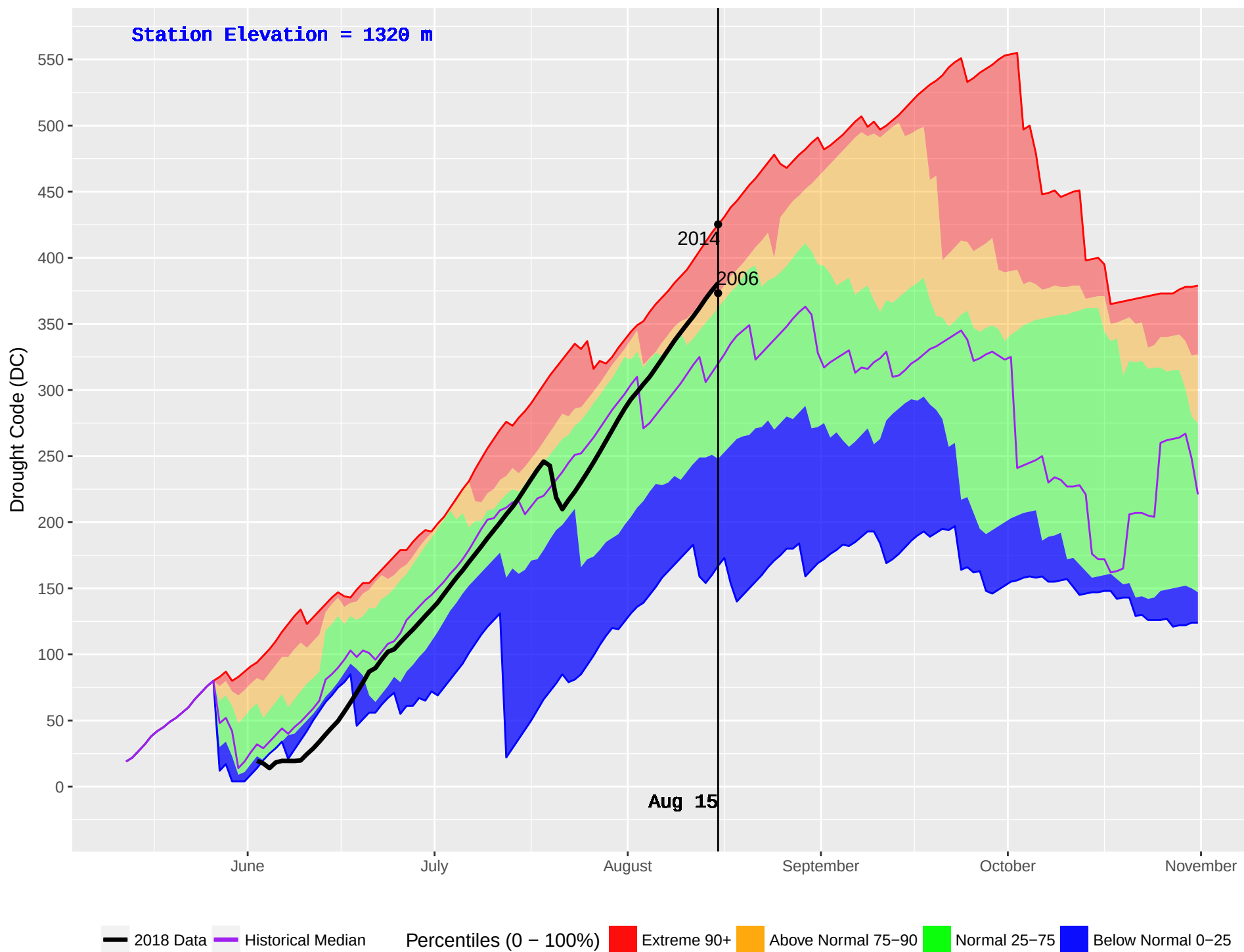
PINE CREEK (938) : Historical (2006–2016) and Current (2018) Daily Drought Code (DC)
