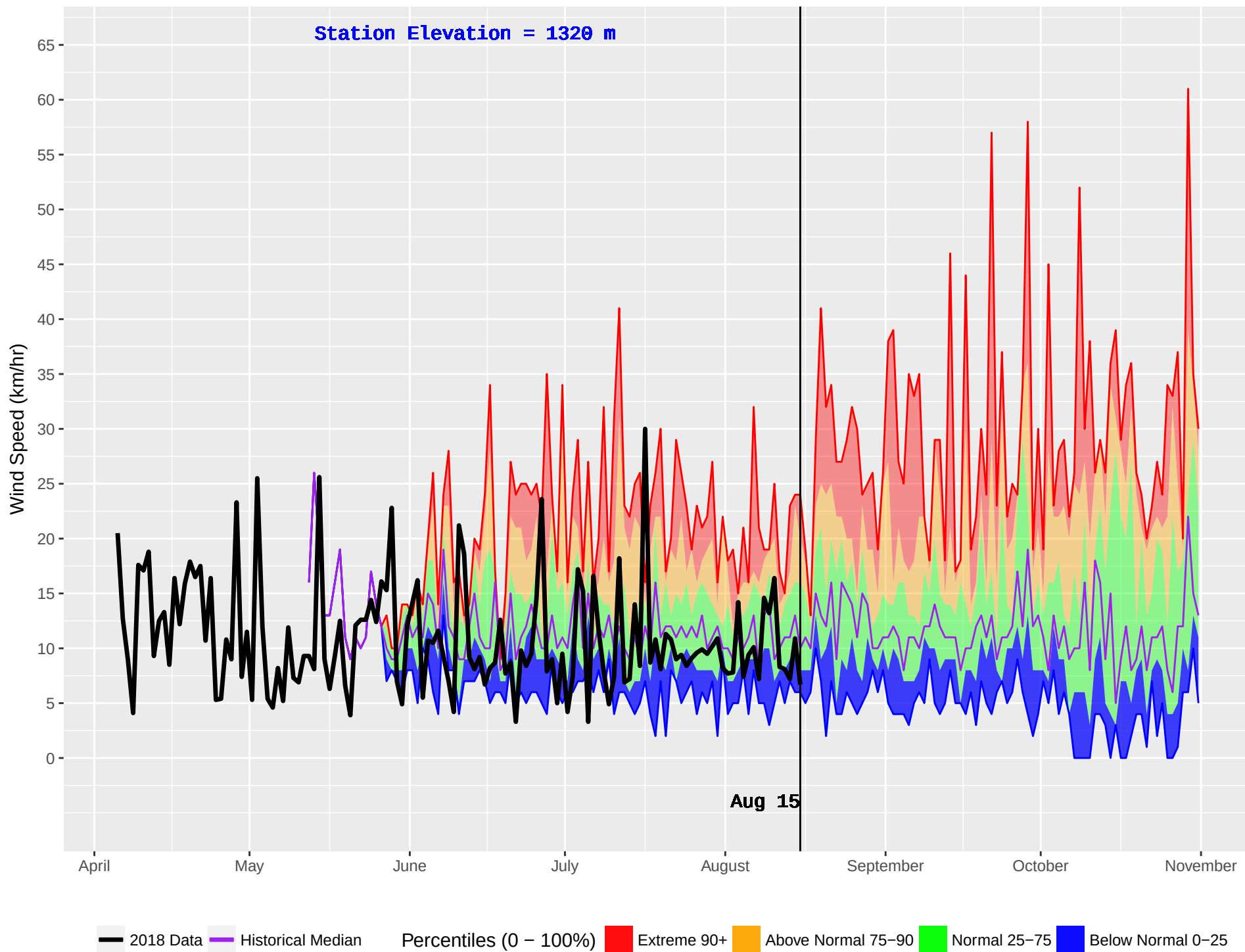
PINE CREEK (938) : Historical (2006–2016) and Current (2018) Daily Wind Speed
